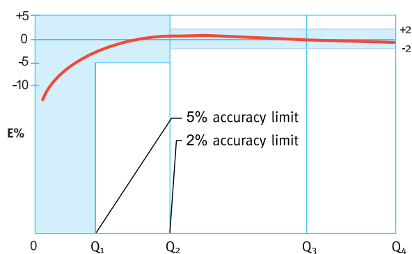
Accuracy Curve
